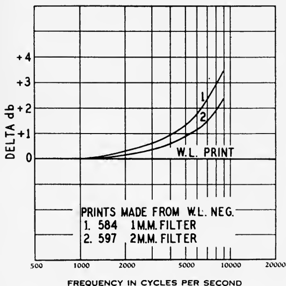
FIG. 11. Net improvement in high-frequency response of ultraviolet prints over white-light prints.
